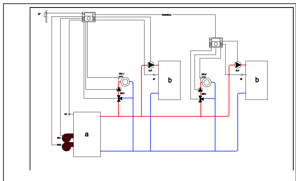
a Boiler
